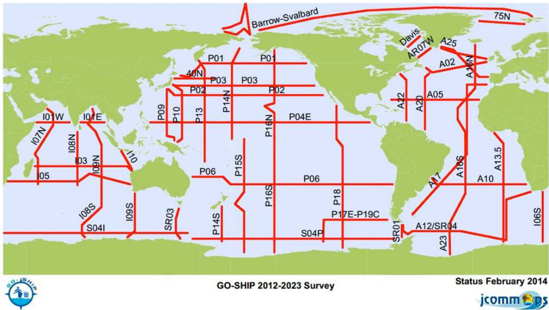
Figure 4. Map of GO-SHIP Repeat Hydrographic Surveys; current status as of February 2014. Source: .
