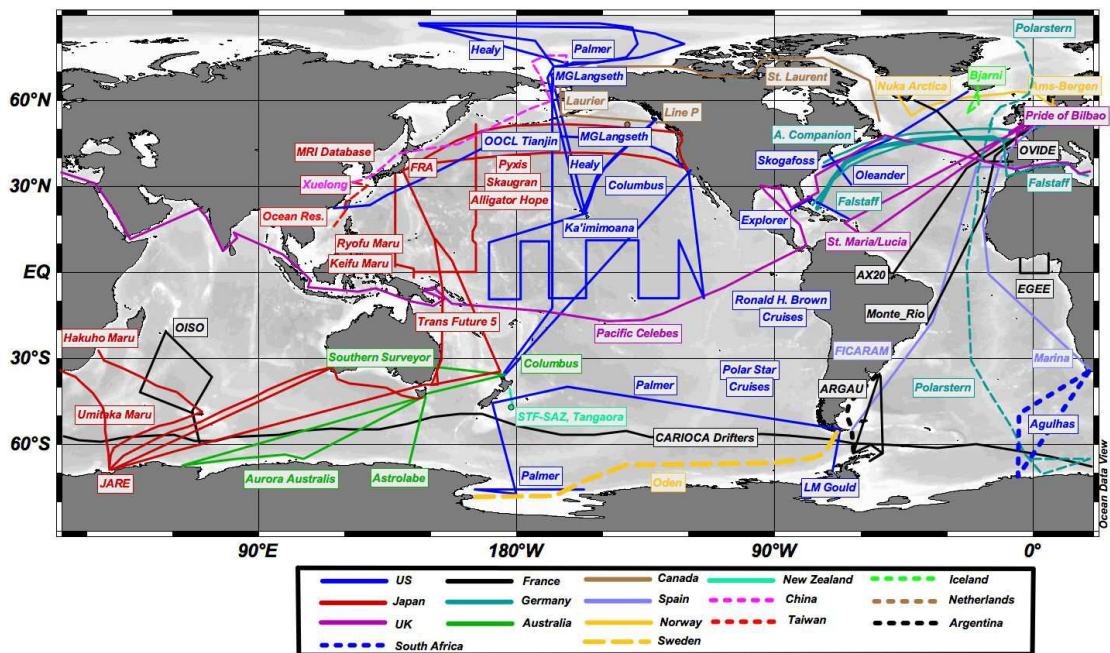
Figure 5. Map of global ship of opportunity/CO 2 cruise tracks for underway measurements, current status as of March 2014. Source: .
